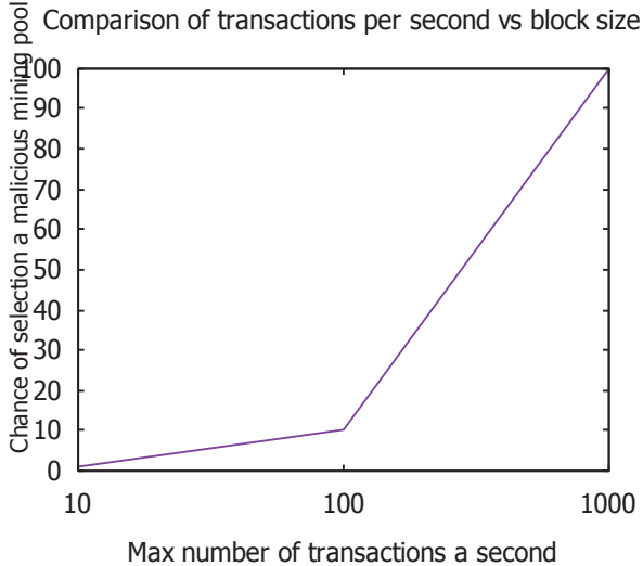
Figure 3: Graph showing relationship between block size and transactions a second
